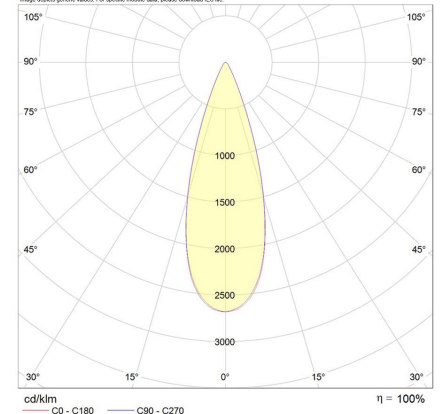
*Albi 7W/13W/18W 30°
