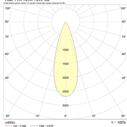
*Albi 7W/13W/18W 30°
