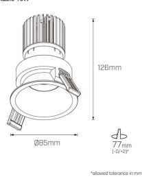
Albi Maxi Adjustable 13W
