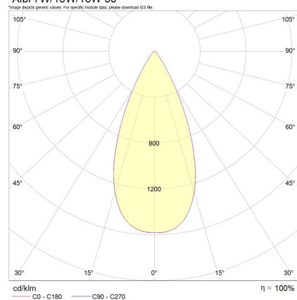
*Albi 7W/13W/18W 50°
