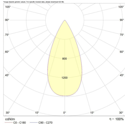
*Albi 7W/13W/18W 50°
