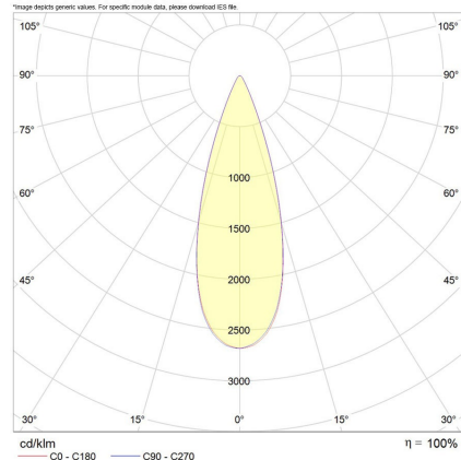
*Albi 7W/13W/18W 30°
