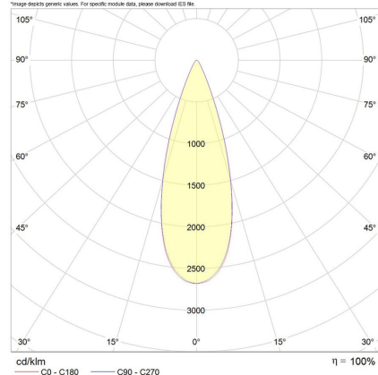
*Bron 7W/13W/18W 30°
