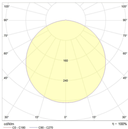
Neonflex Side Bendable 120°
